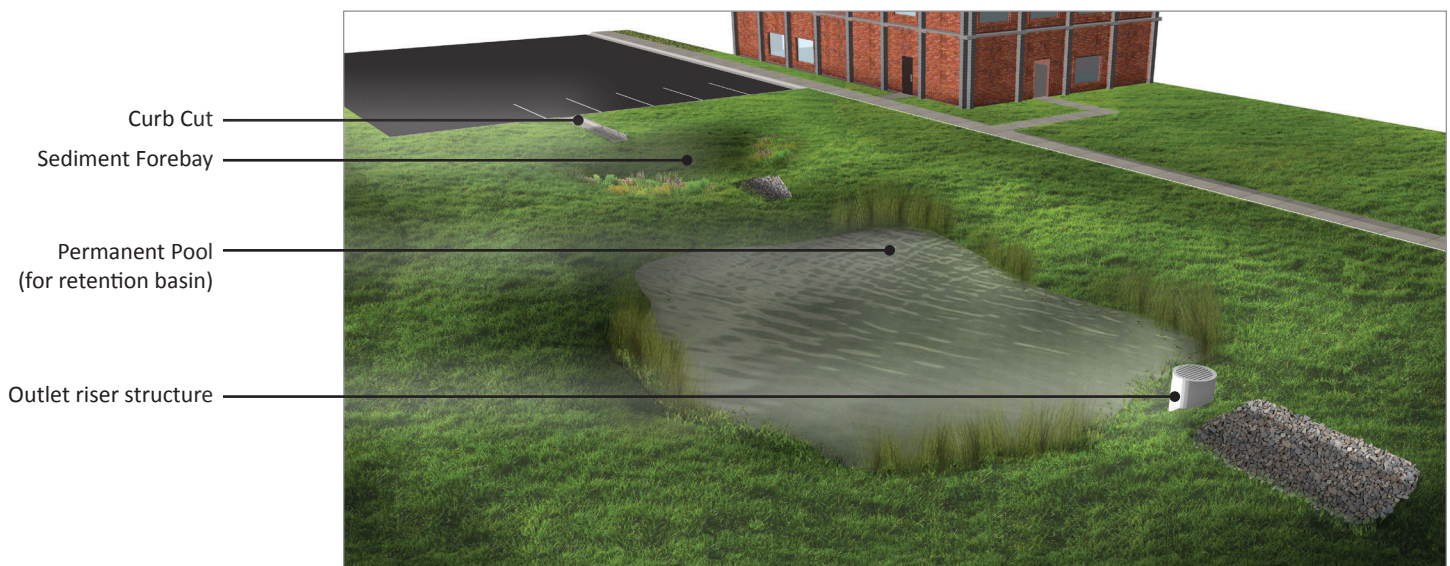
Illustration of a retention basin (permanent pool of water) to capture runoff from adjacent parking lot and in some instances, the adjacent building
