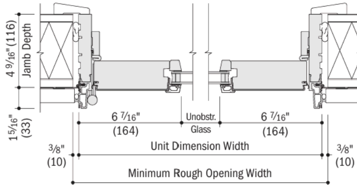
Horizontal Section
